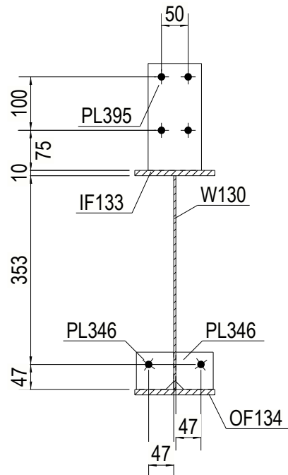
SEC A 1:10
